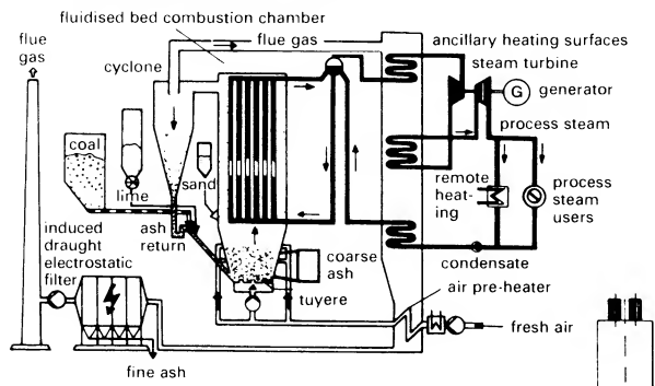
2 Scheme for a power station with heat/power coupling
